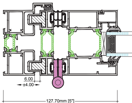
Outerframe detail with adjustable jambs
